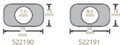
Drawings illustrate Nominal Proximal Internal Dimensions and Minimum Internal Diameter (I.D.), NOT TO SCALE.
